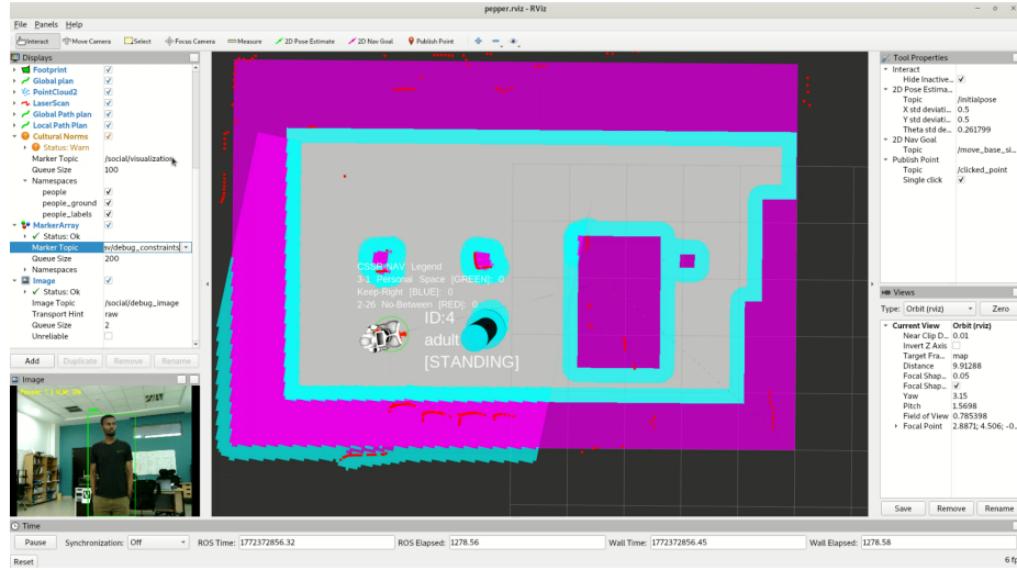
Fig. 4: Elder status detection and representation of a person the dynamic local cost map.
