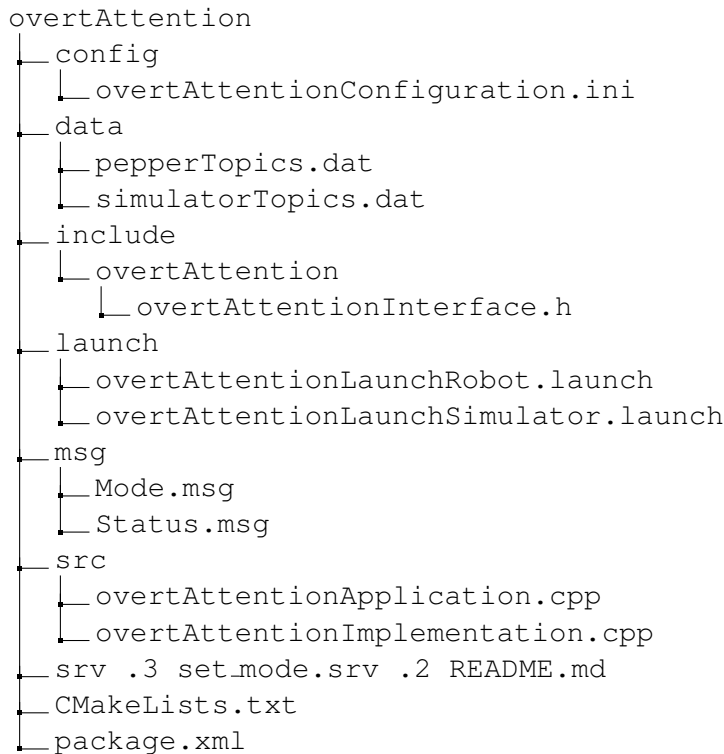
Figure 1: File structure for overtAttention node
