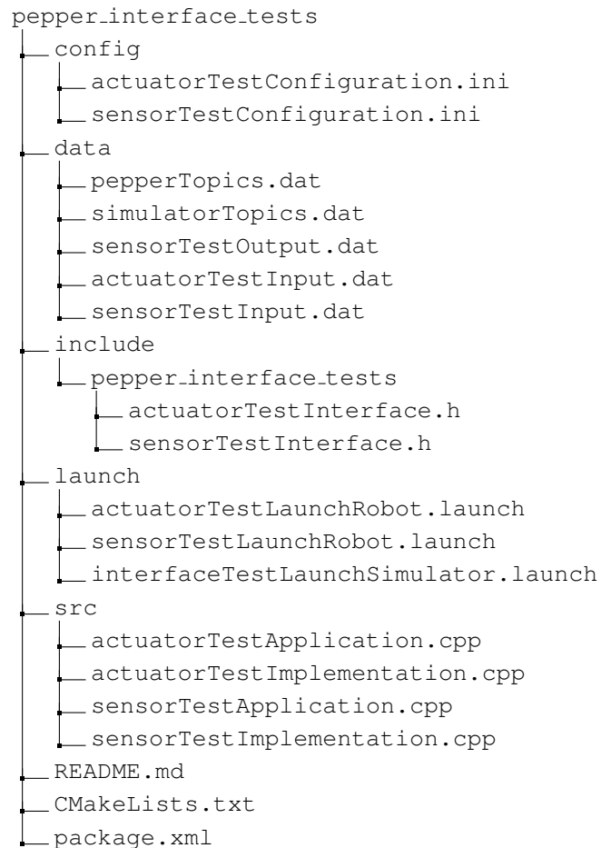
Figure 5: Directory structure for the pepper_interface_tests package. There are two nodes: actuatorTest and sensorTest .
